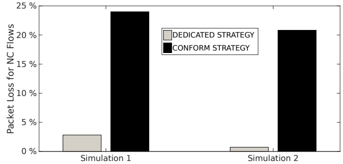
Figure 5. Packet Loss for Non Conformant Flows
