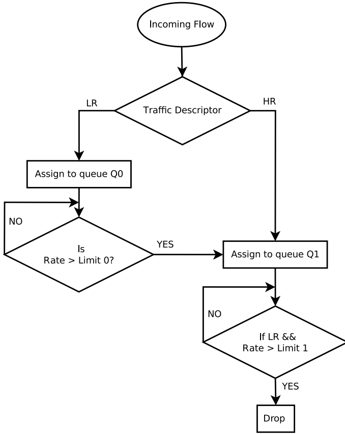
Figure 3. Strategy Flowchart
